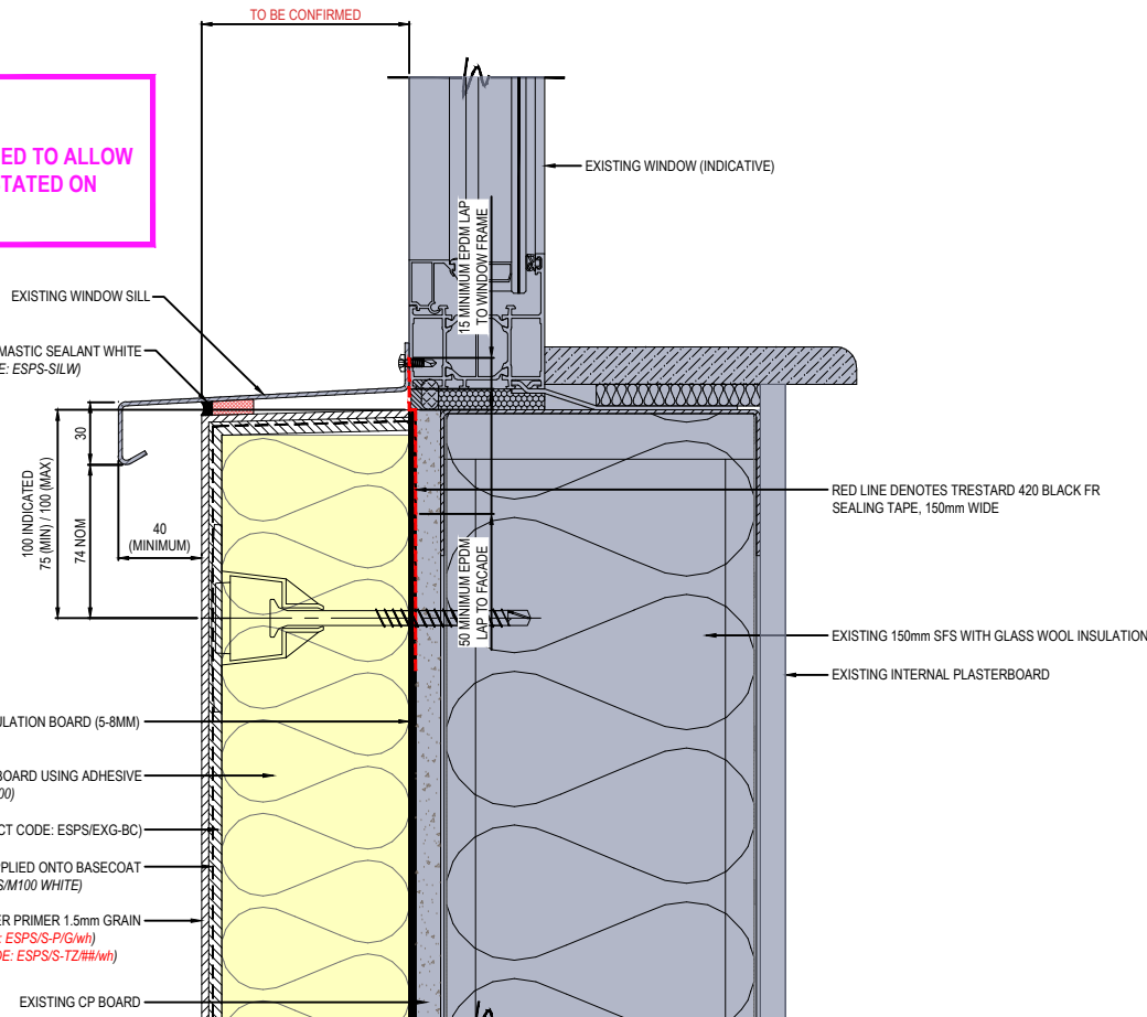
03 CROSS SECTION - RENDER / WINDOW SILL INTERFACE DETAIL Scale 1:2
