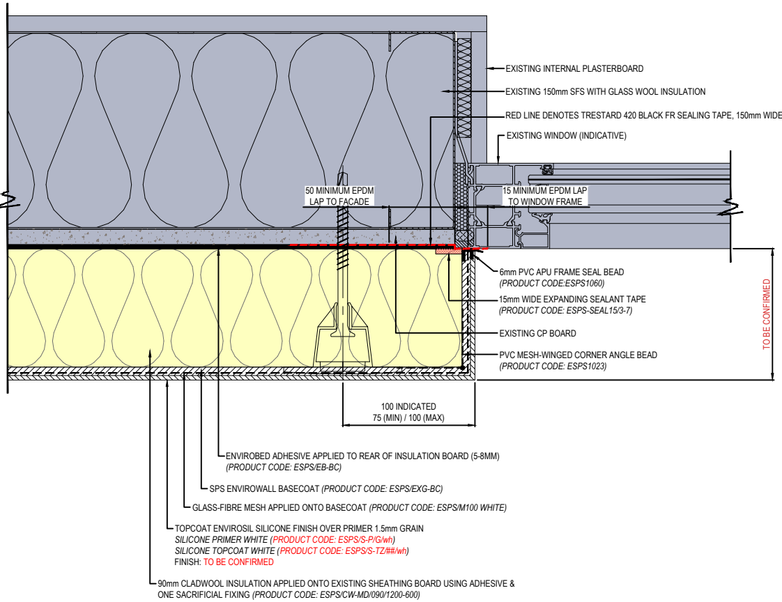
01 PLAN SECTION - RENDER / WINDOW JAMB INTERFACE DETAIL Scale 1:2
